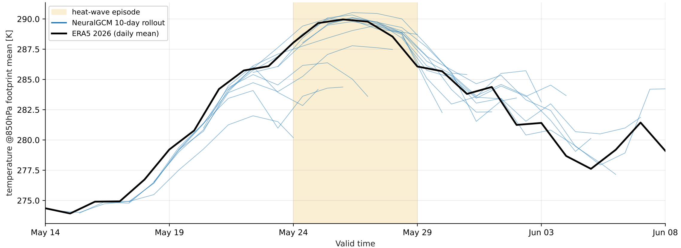
Europe heat-wave 2026-05-24..2026-05-29 — footprint-mean temperature @ 850 hPa (mixture, > p99)
