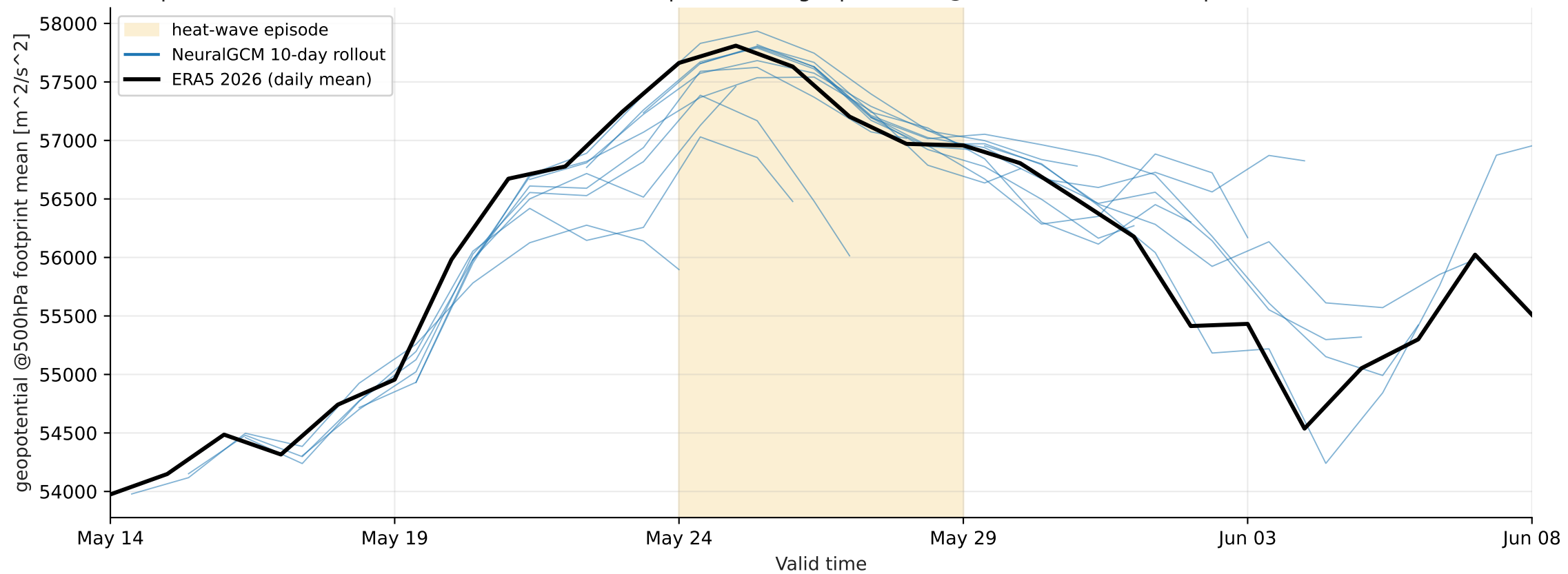
Europe heat-wave 2026-05-24..2026-05-29 — footprint-mean geopotential @ 500 hPa (mixture, > p99)
