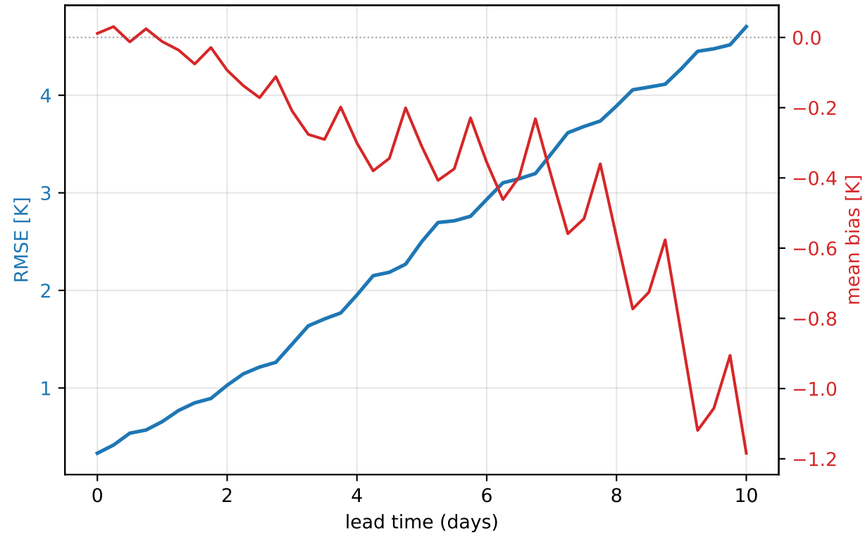
Europe heat-wave 2026-06-22..2026-07-24 — footprint temperature@850 hPa (mean of 19 rollouts)
