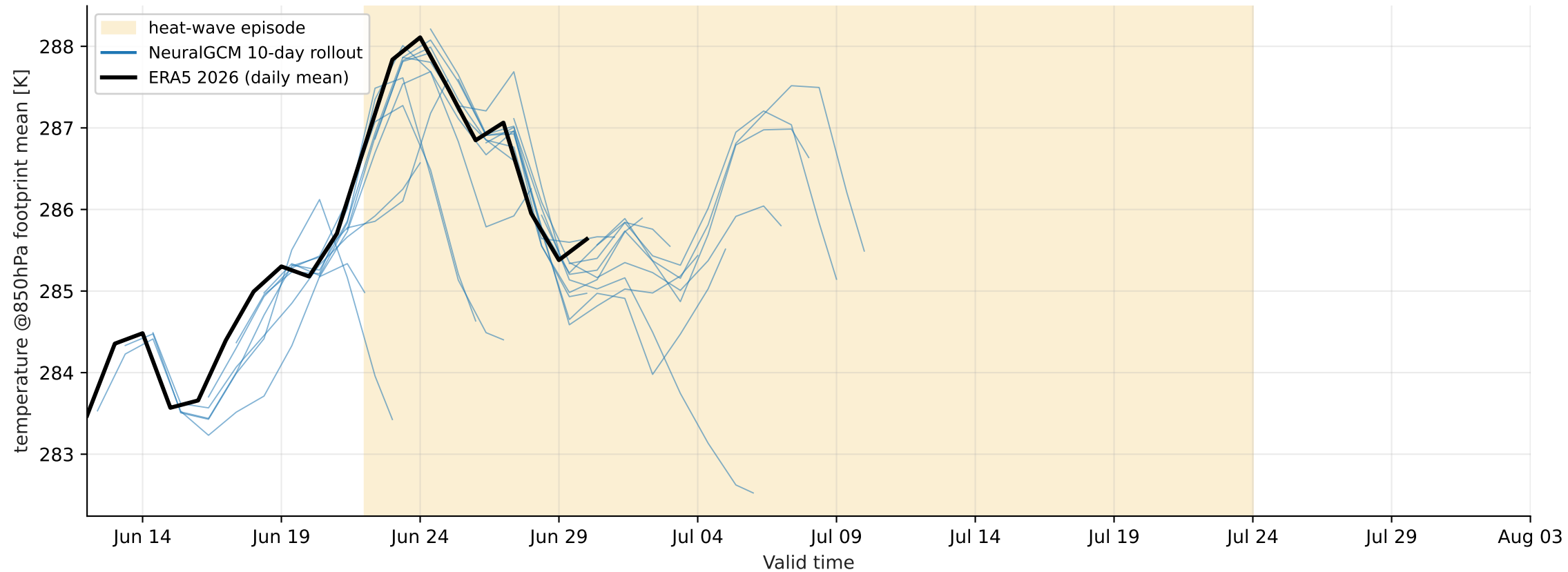
Europe heat-wave 2026-06-22..2026-07-24 — footprint-mean temperature @ 850 hPa (mixture, > p99)
