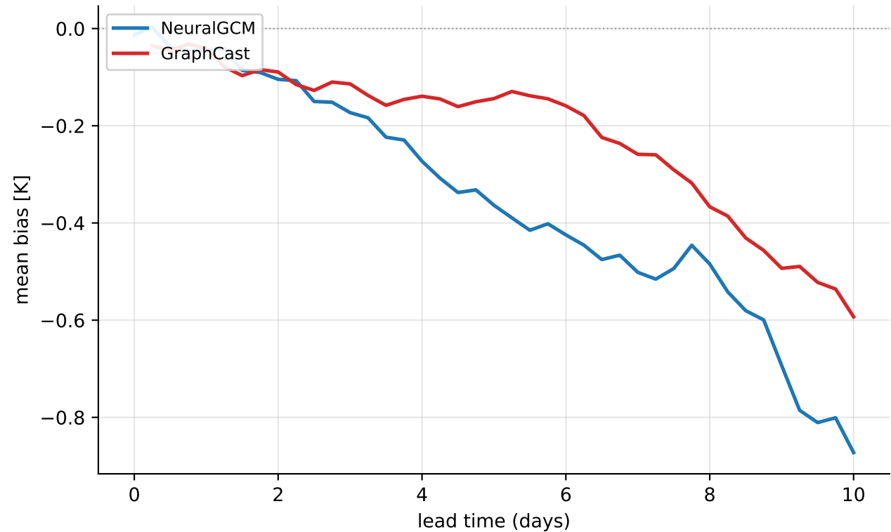
temperature@850 hPa — mean bias over all cordex heat waves (9 events, > p99)
