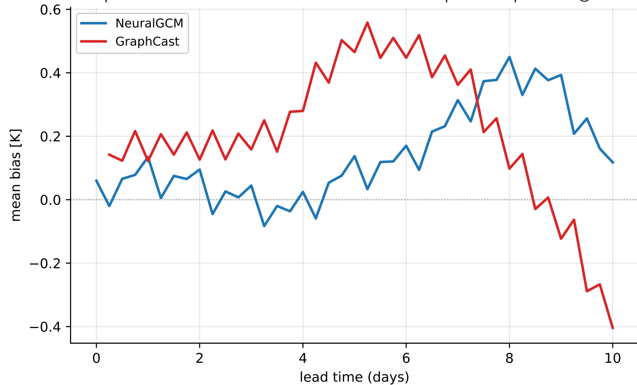
Europe heat-wave 2023-07-08..2023-07-26 — footprint temperature@850 hPa (mean of 29 rollouts)
