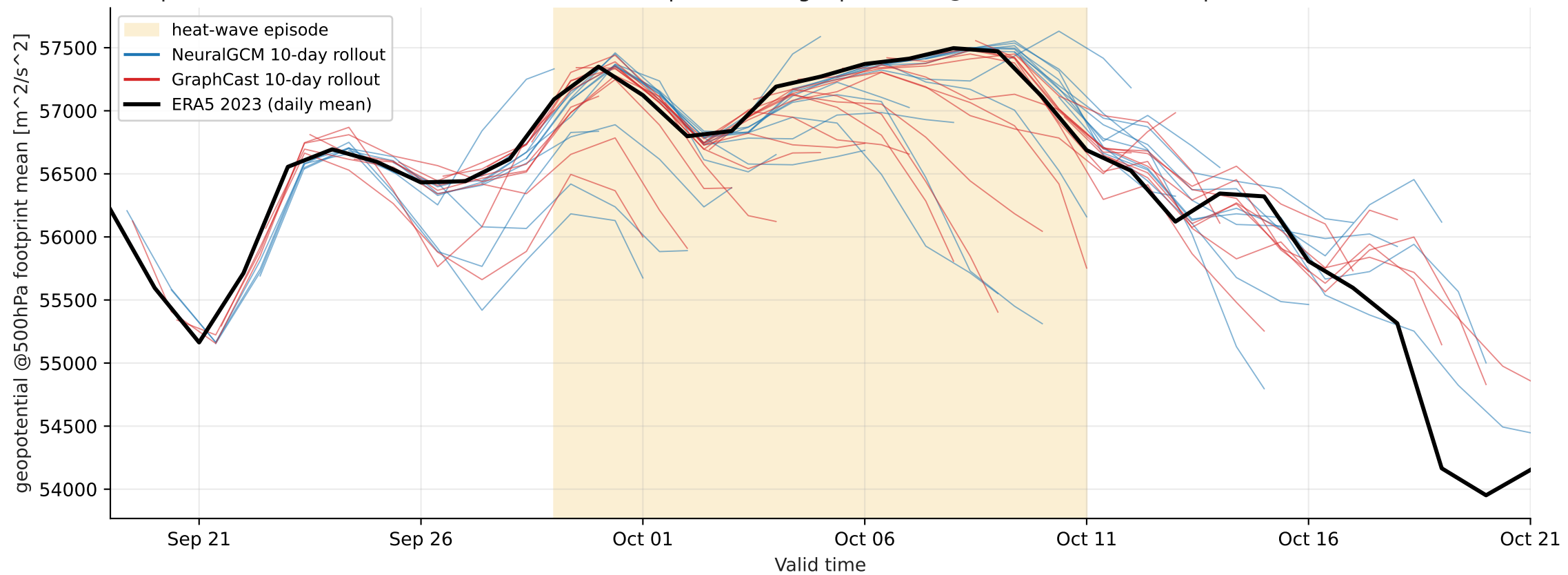
Europe heat-wave 2023-09-29..2023-10-11 — footprint-mean geopotential @ 500 hPa (mixture, > p99)
