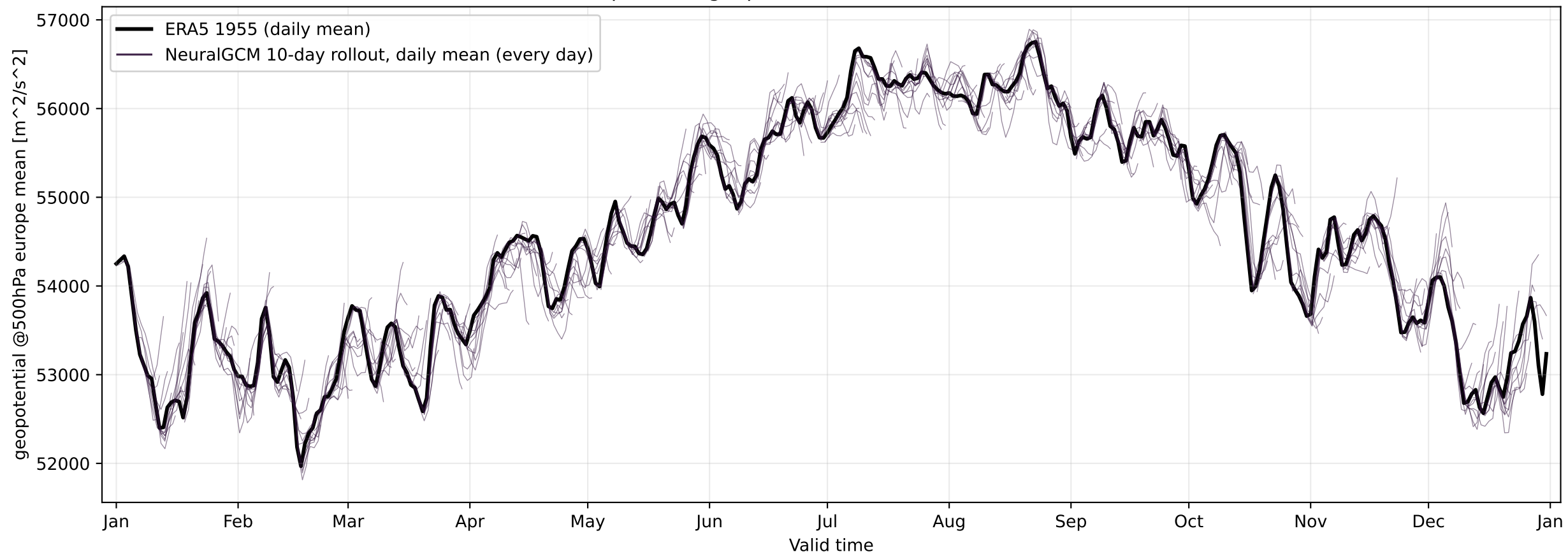
Europe-mean geopotential at 500 hPa — ERA5 1955
