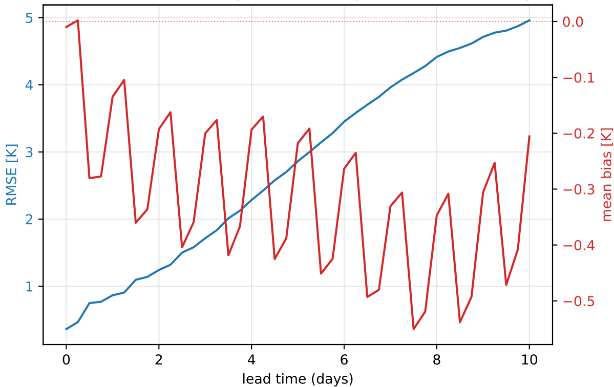
ERA5 1955 — 850 hPa temperature (europe, mean of 355 daily inits)
