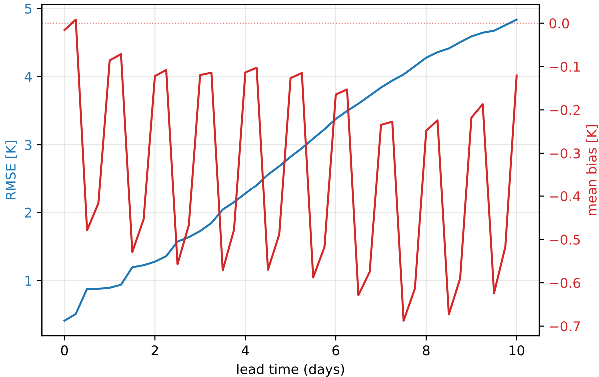
ERA5 1955 — 900 hPa temperature (europe, mean of 355 daily inits)
