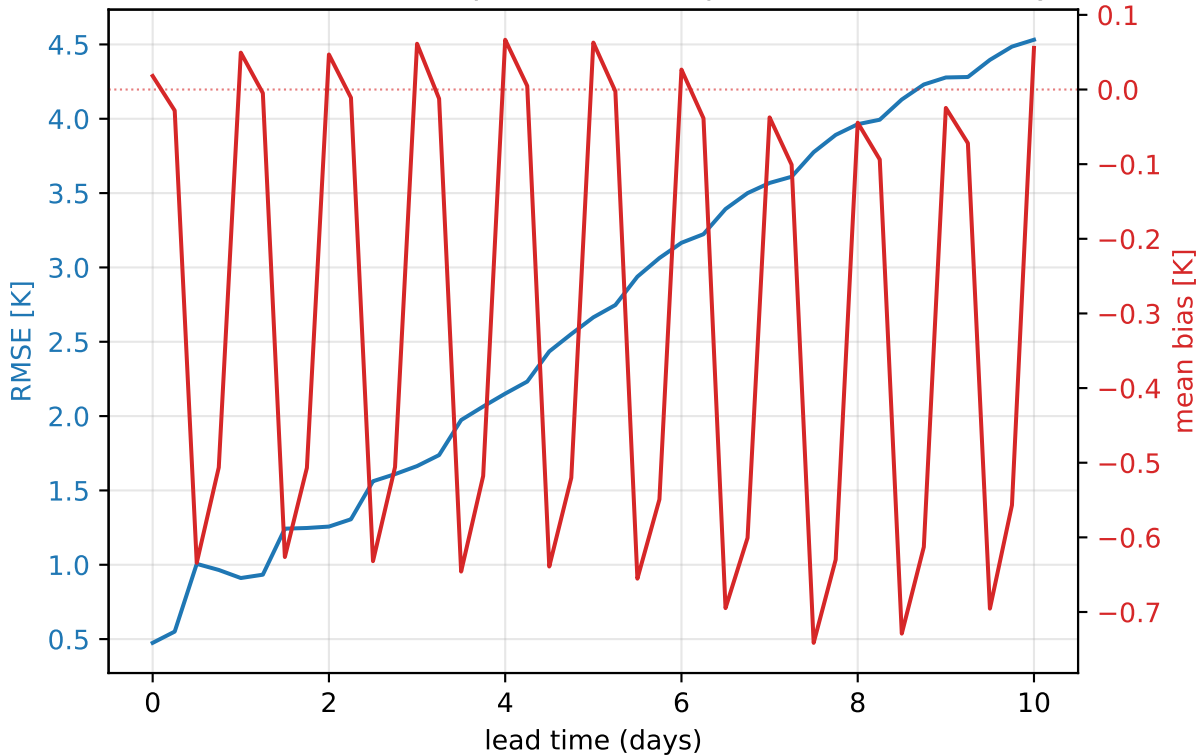
ERA5 1955 — 950 hPa temperature (europe, mean of 355 daily inits)
