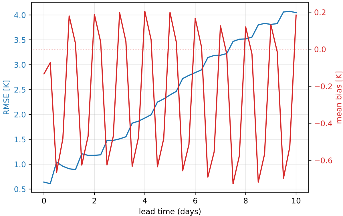
ERA5 1955 — 1000 hPa temperature (europe, mean of 355 daily inits)
