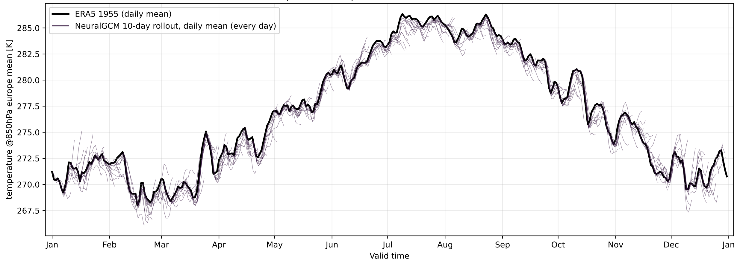
Europe-mean temperature at 850 hPa — ERA5 1955
