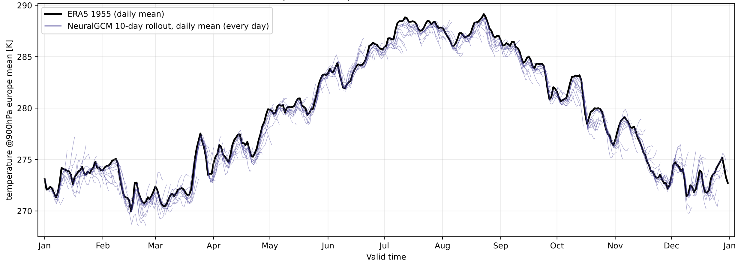
Europe-mean temperature at 900 hPa — ERA5 1955
