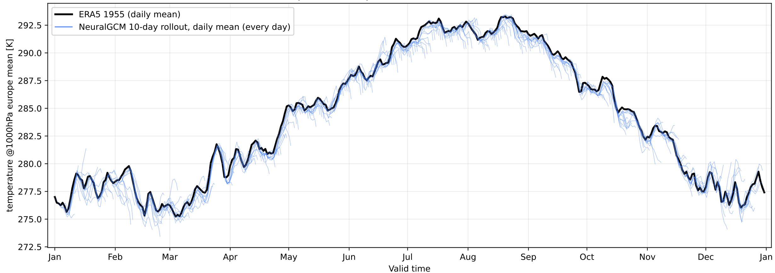
Europe-mean temperature at 1000 hPa — ERA5 1955
