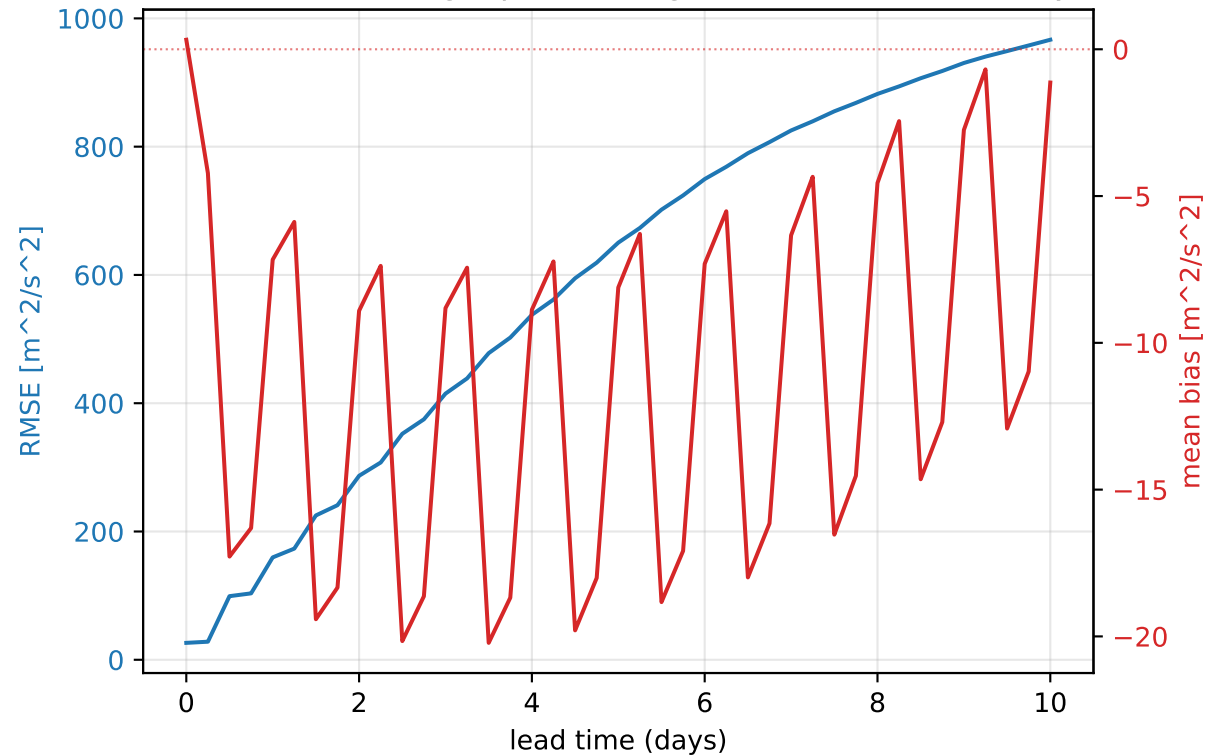
ERA5 1955 — 500 hPa geopotential (global, mean of 355 daily inits)
