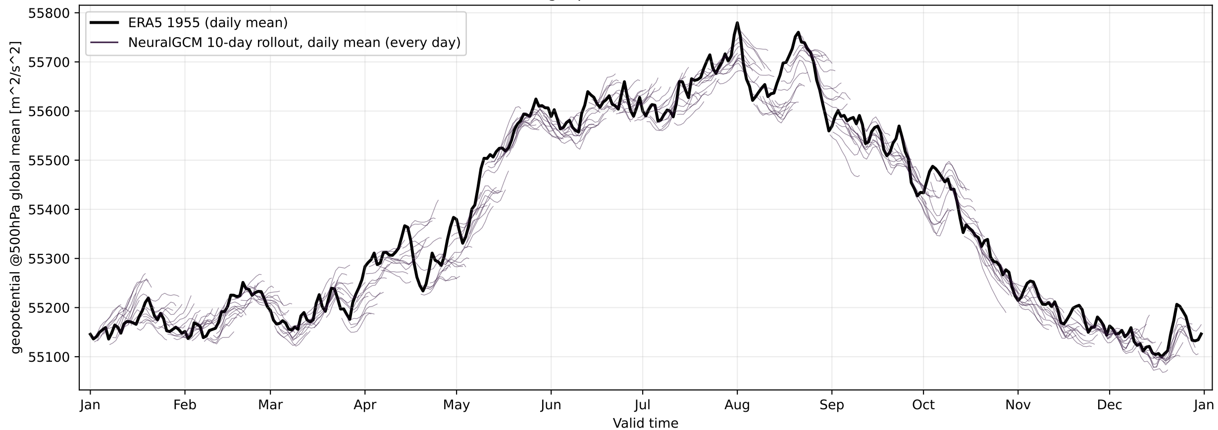
Global-mean geopotential at 500 hPa — ERA5 1955
