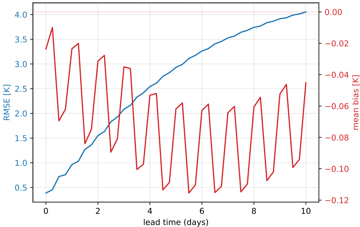
ERA5 1955 — 900 hPa temperature (global, mean of 355 daily inits)
