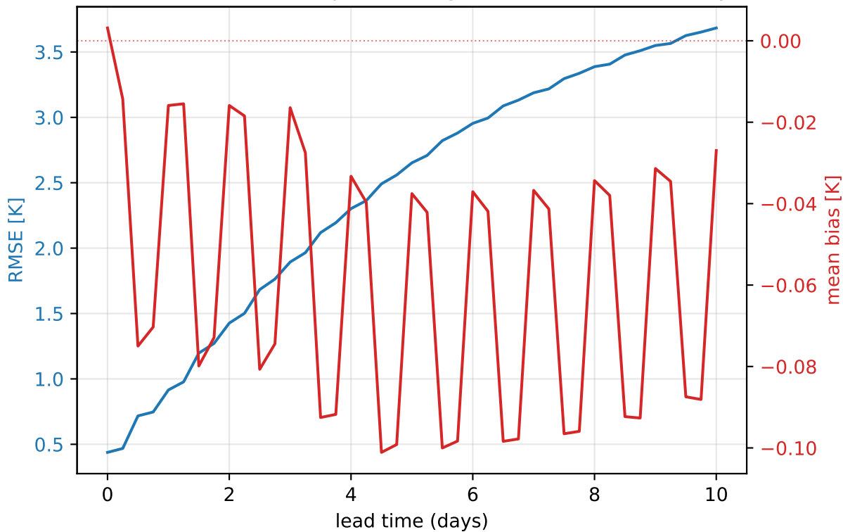
ERA5 1955 — 950 hPa temperature (global, mean of 355 daily inits)
