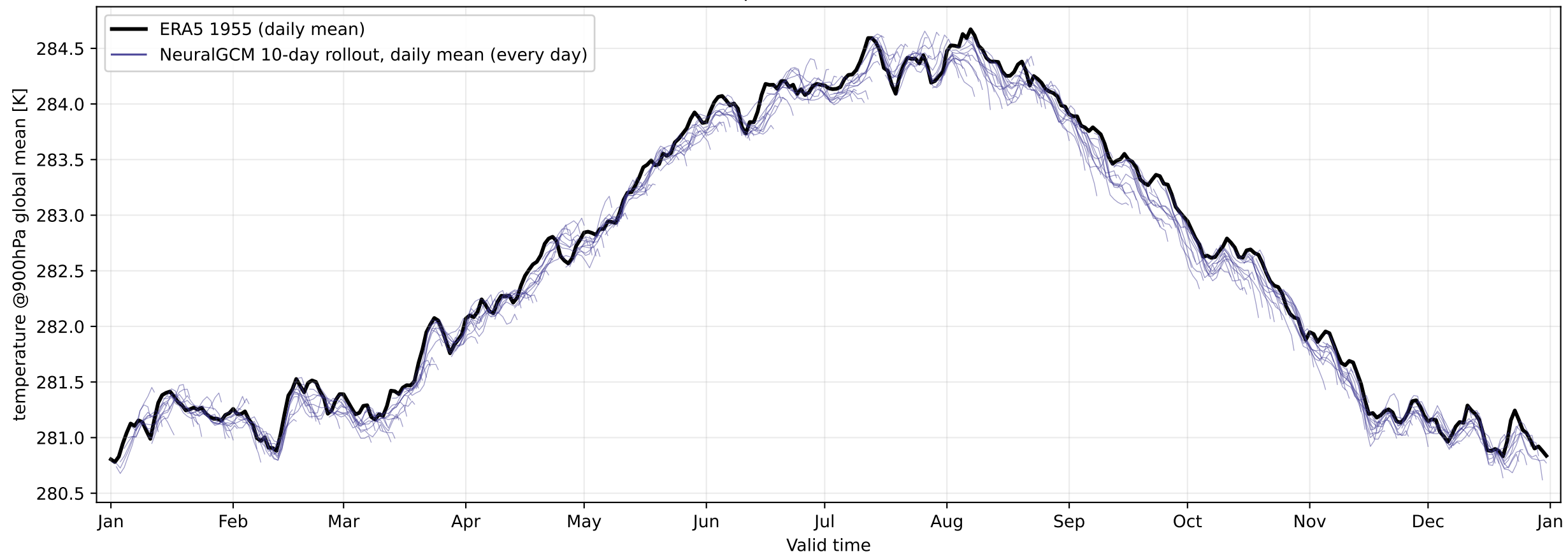
Global-mean temperature at 900 hPa — ERA5 1955
