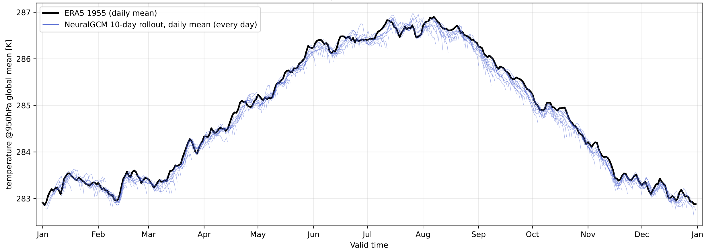
Global-mean temperature at 950 hPa — ERA5 1955
