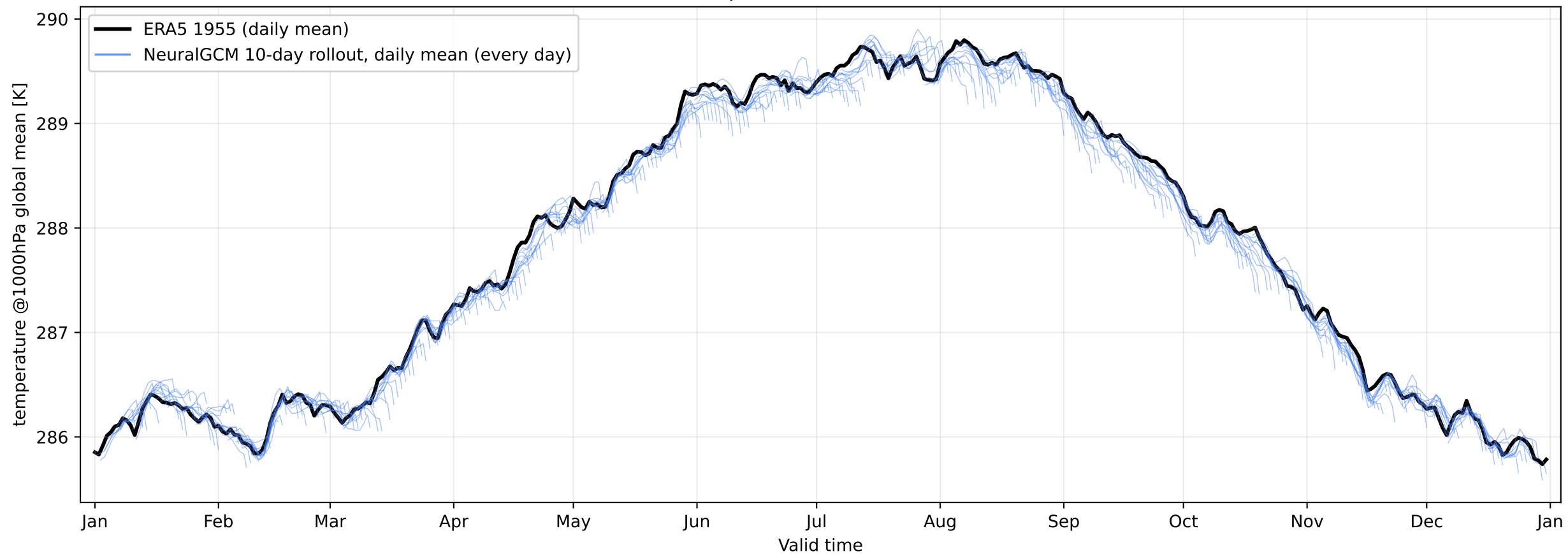
Global-mean temperature at 1000 hPa — ERA5 1955
