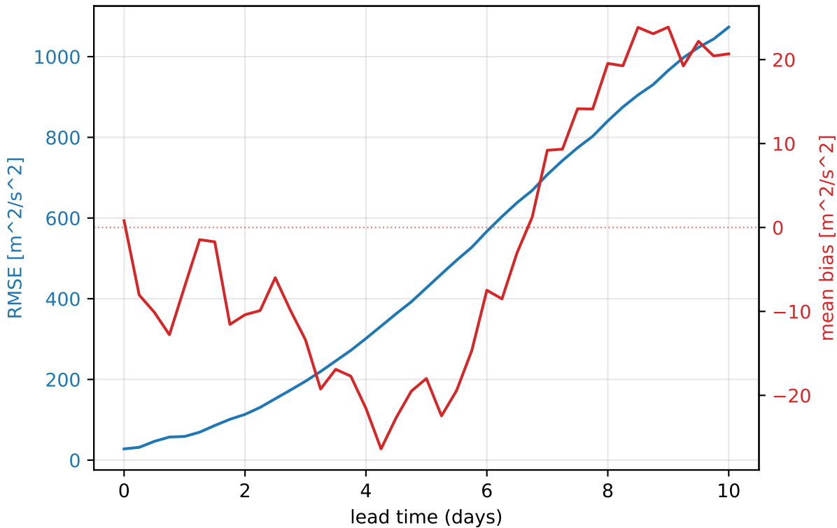
ERA5 2023 — 500 hPa geopotential (europe, mean of 355 daily inits)
