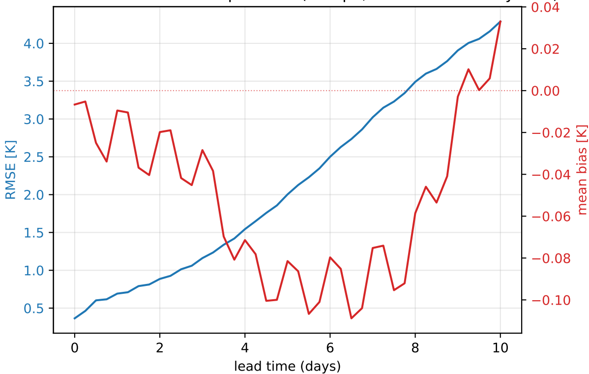
ERA5 2023 — 850 hPa temperature (europe, mean of 355 daily inits)
