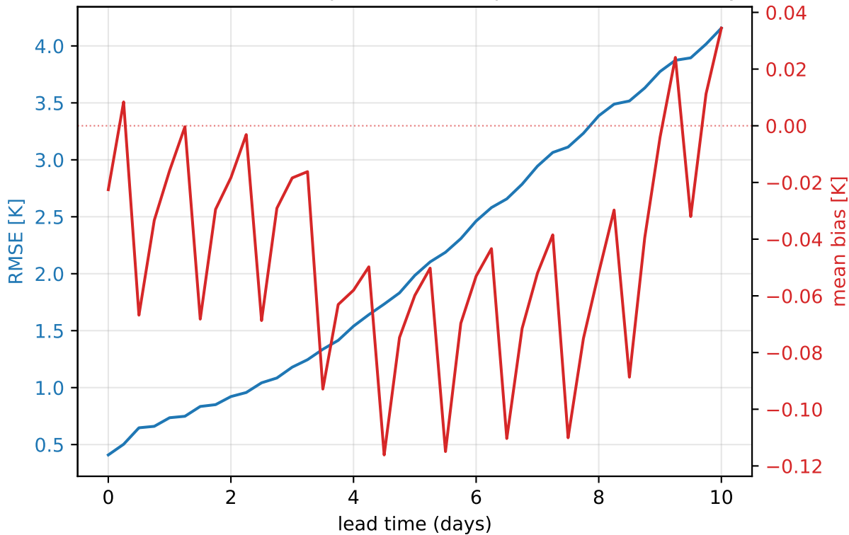
ERA5 2023 — 900 hPa temperature (europe, mean of 355 daily inits)
