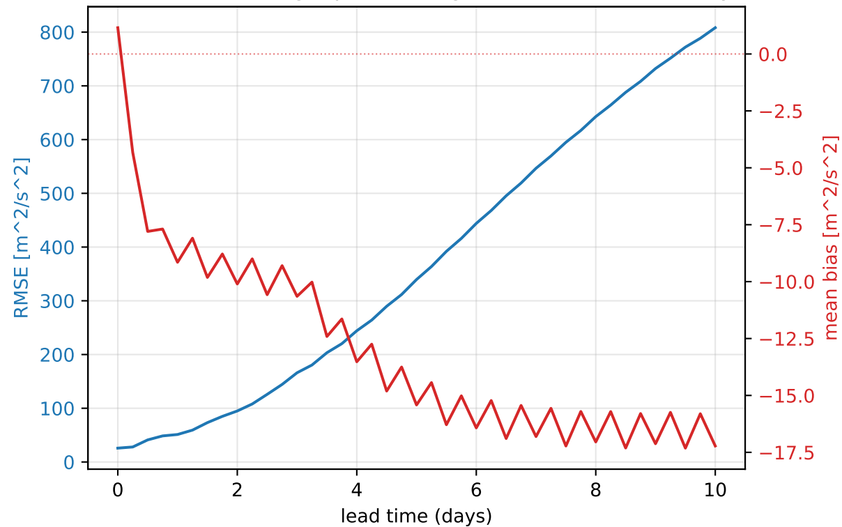
ERA5 2023 — 500 hPa geopotential (global, mean of 355 daily inits)
