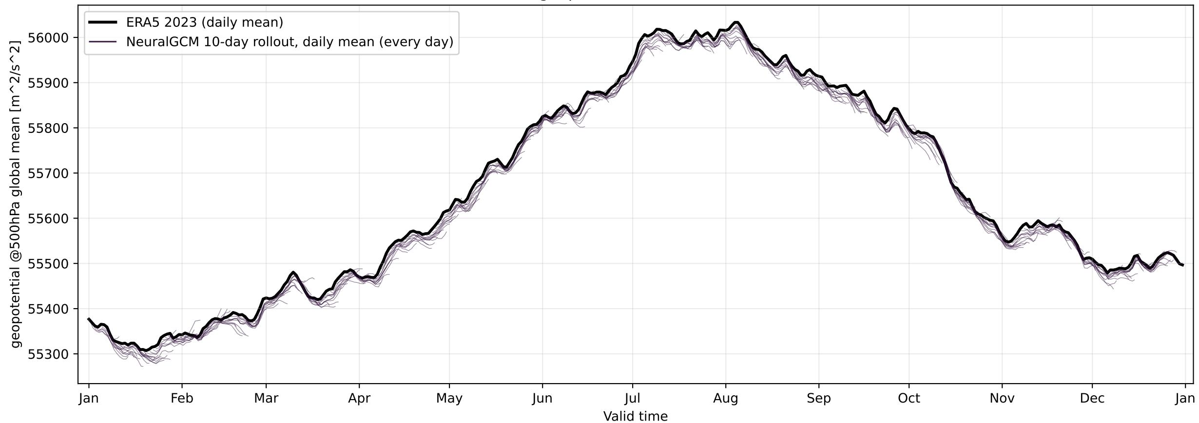
Global-mean geopotential at 500 hPa — ERA5 2023
