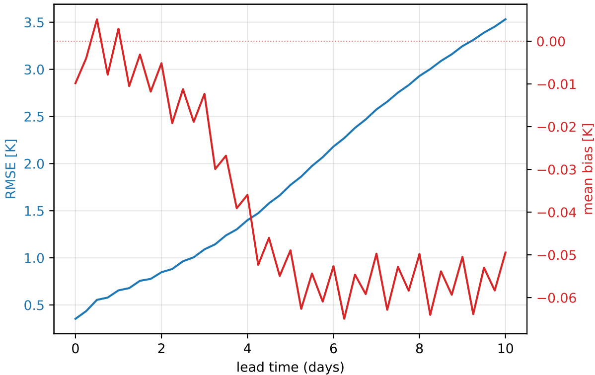
ERA5 2023 — 850 hPa temperature (global, mean of 355 daily inits)
