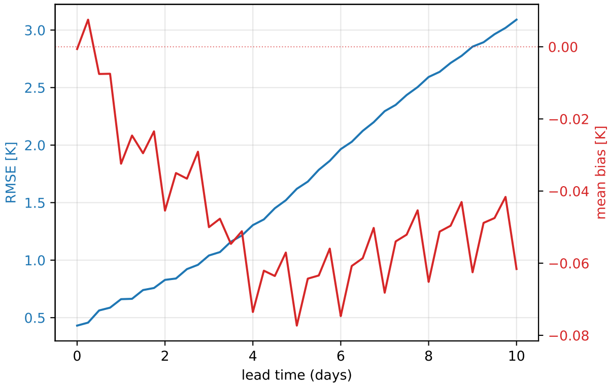
ERA5 2023 — 950 hPa temperature (global, mean of 355 daily inits)
