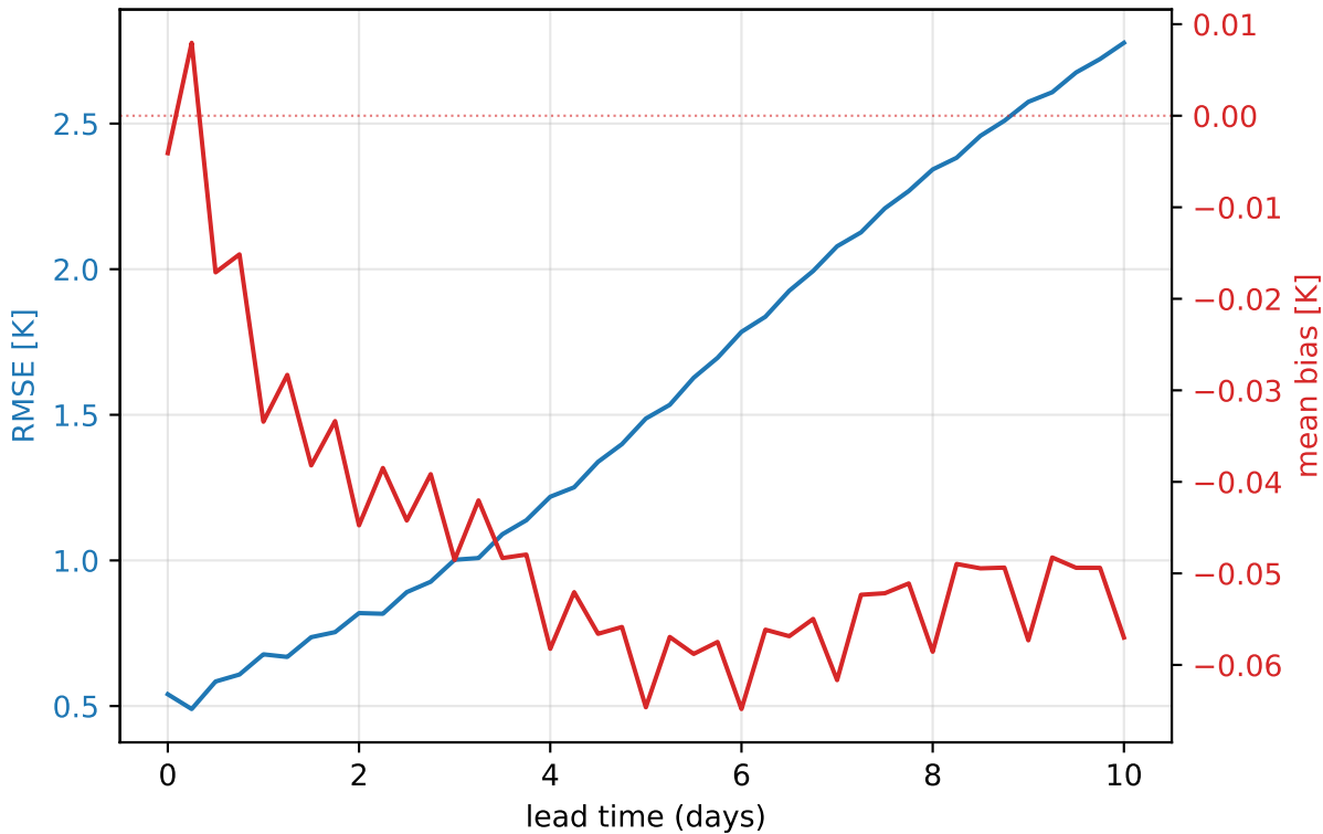
ERA5 2023 — 1000 hPa temperature (global, mean of 355 daily inits)
