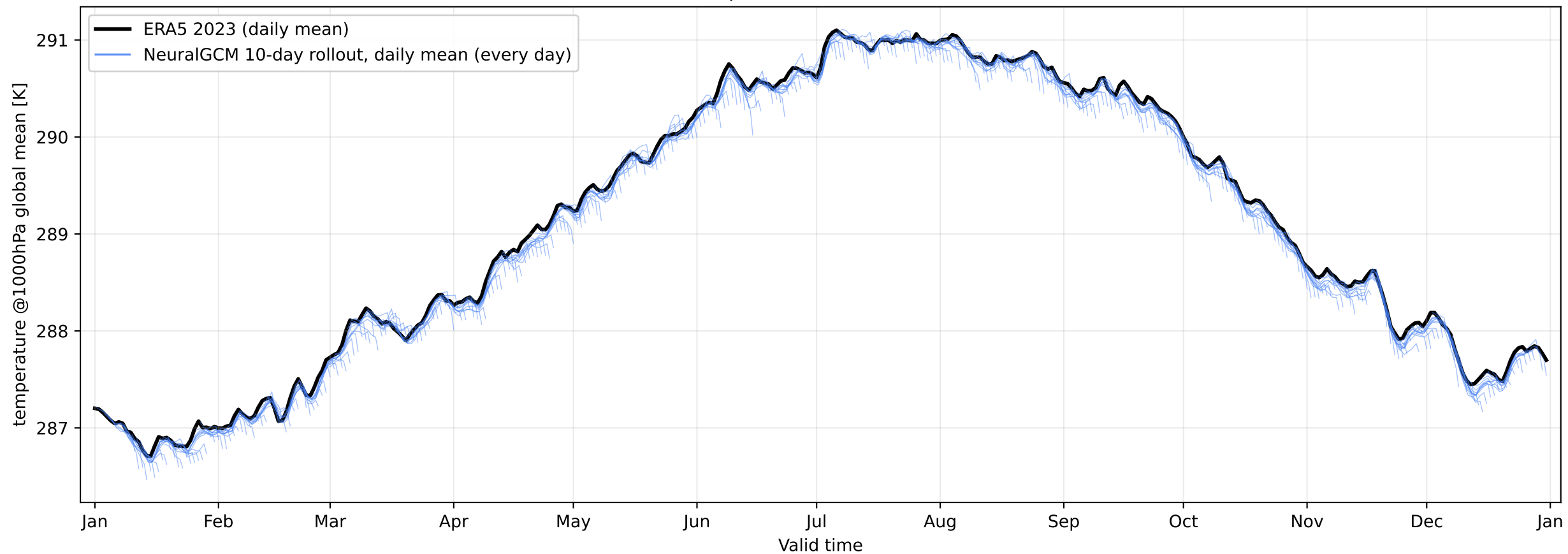
Global-mean temperature at 1000 hPa — ERA5 2023
