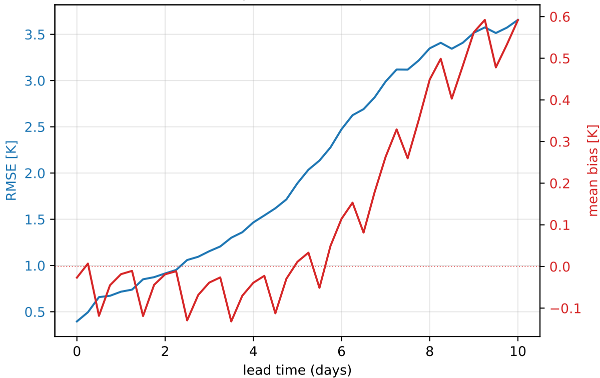
ERA5 2023 — 900 hPa temperature (europe, mean of 31 daily inits)
