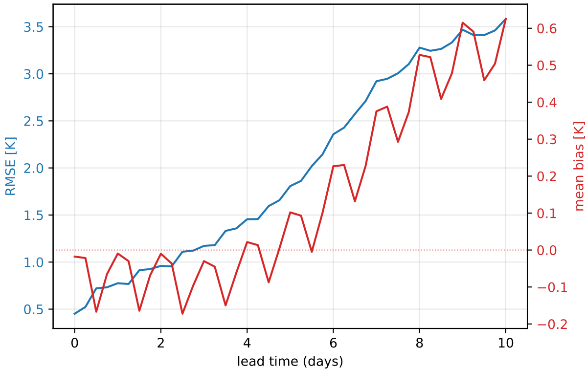
ERA5 2023 — 950 hPa temperature (europe, mean of 31 daily inits)
