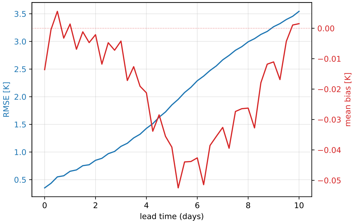
ERA5 2023 — 850 hPa temperature (global, mean of 31 daily inits)
