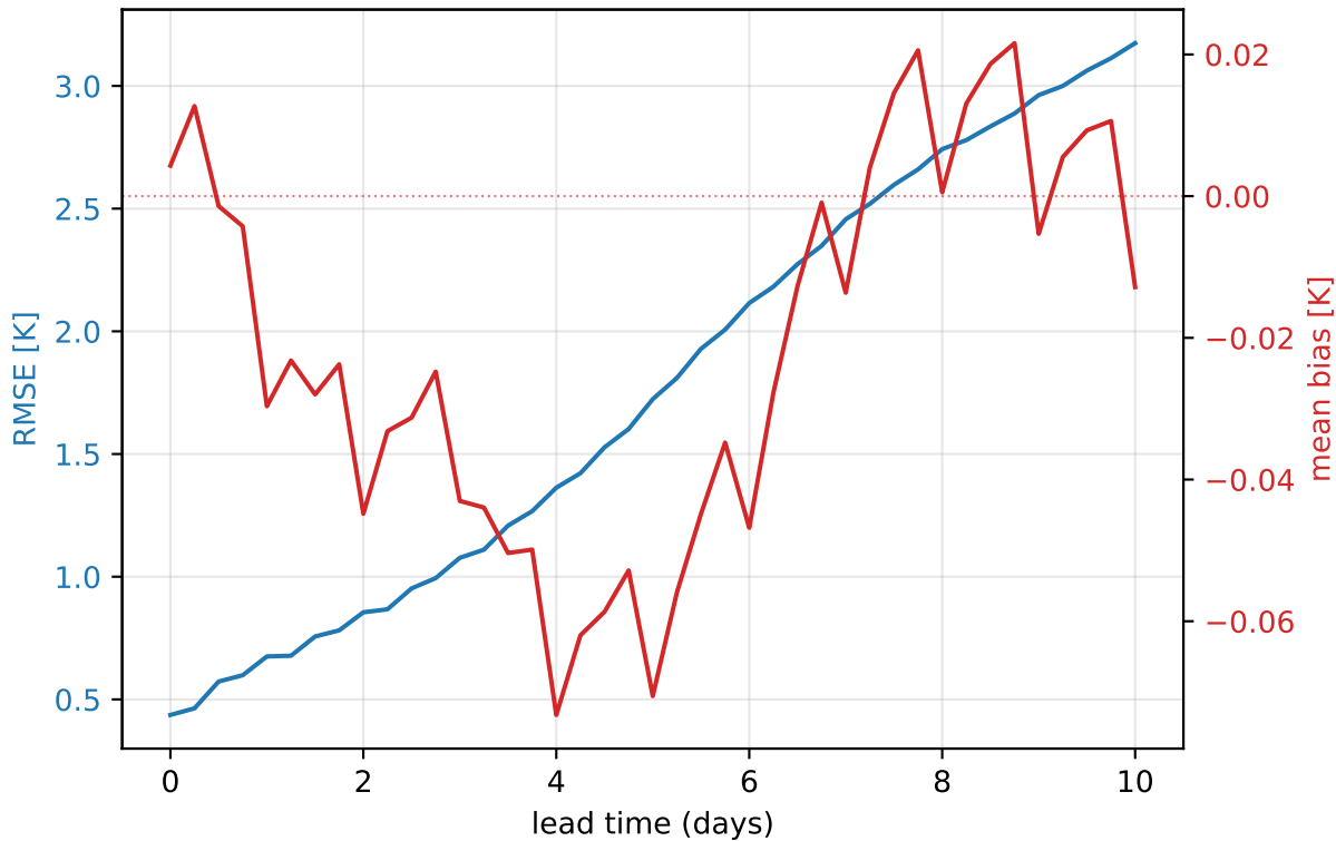
ERA5 2023 — 950 hPa temperature (global, mean of 31 daily inits)
