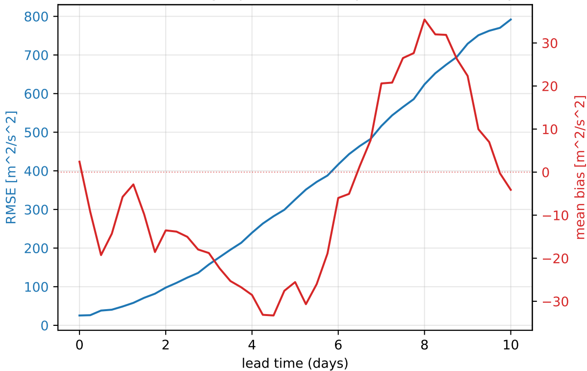
ERA5 2023 — 500 hPa geopotential (europe, mean of 30 daily inits)
