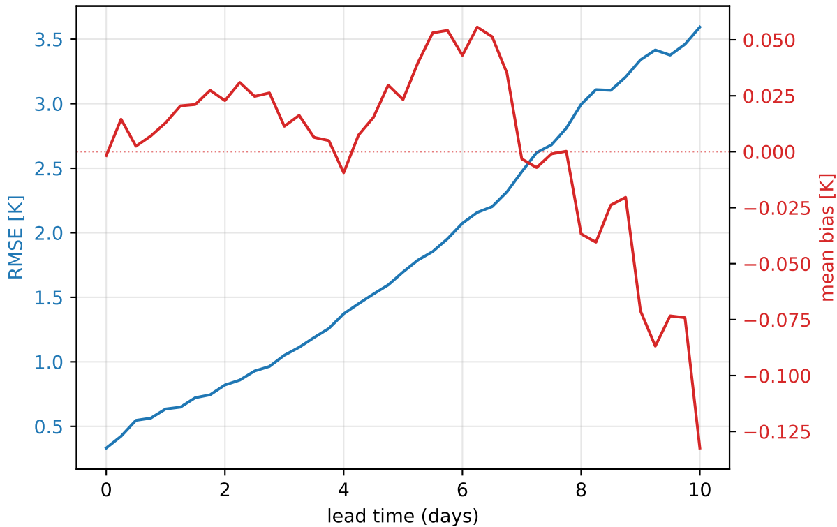
ERA5 2023 — 850 hPa temperature (europe, mean of 30 daily inits)
