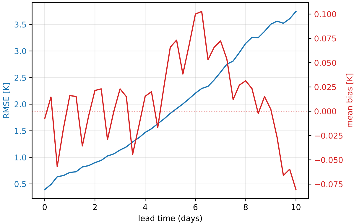
ERA5 2023 — 900 hPa temperature (europe, mean of 30 daily inits)
