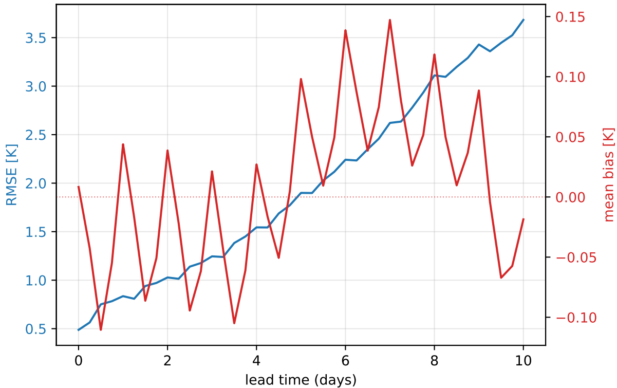
ERA5 2023 — 950 hPa temperature (europe, mean of 30 daily inits)
