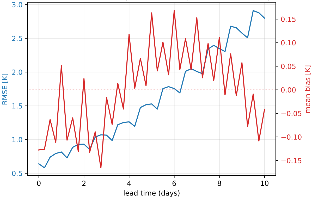
ERA5 2023 — 1000 hPa temperature (europe, mean of 30 daily inits)
