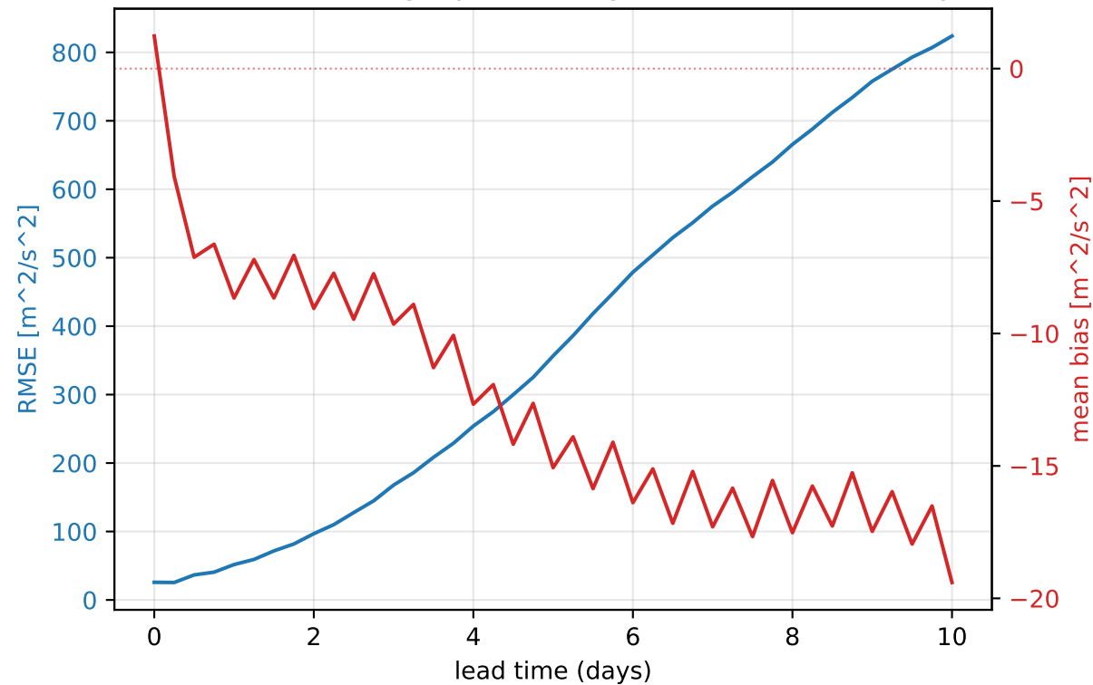
ERA5 2023 — 500 hPa geopotential (global, mean of 30 daily inits)
