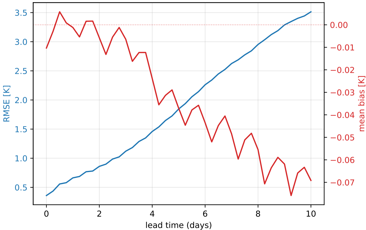
ERA5 2023 — 850 hPa temperature (global, mean of 30 daily inits)
