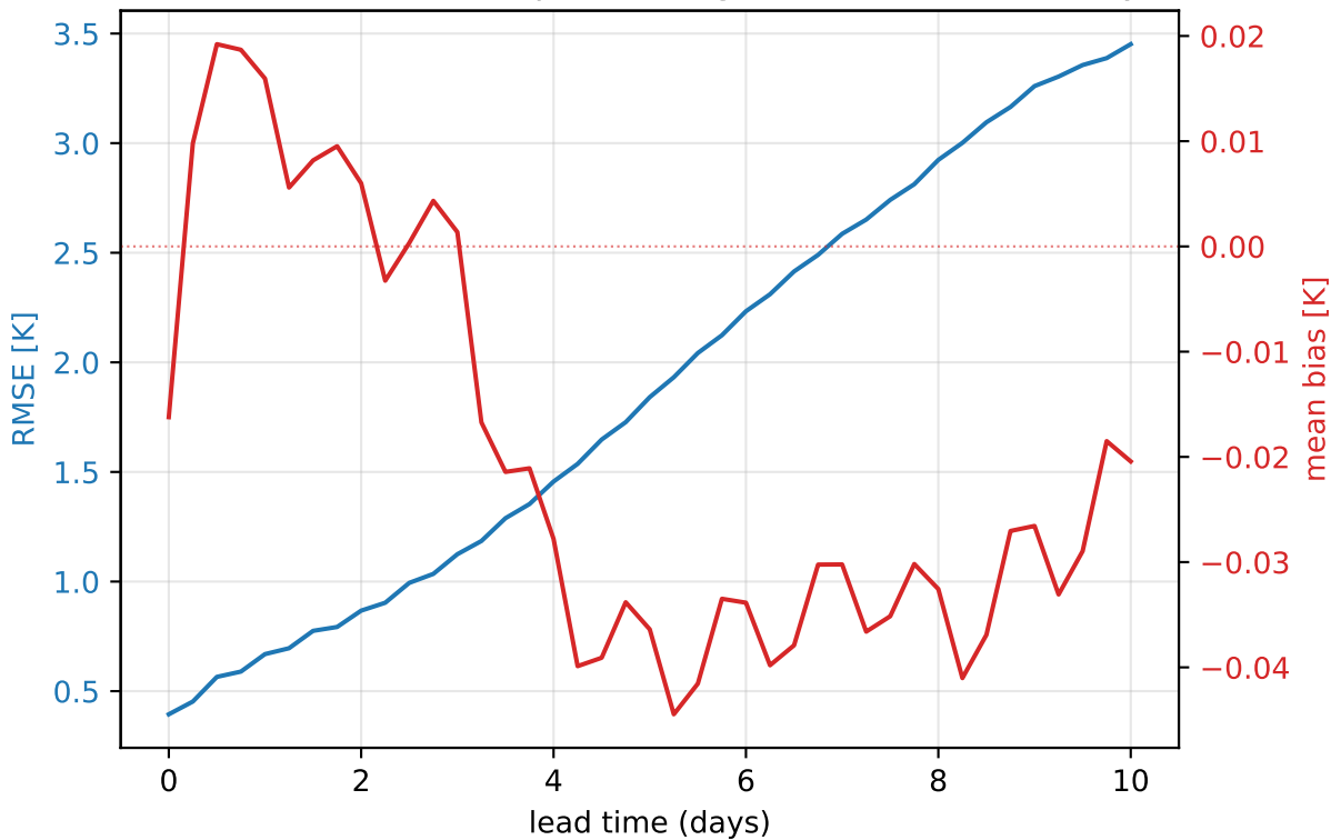
ERA5 2023 — 900 hPa temperature (global, mean of 30 daily inits)
