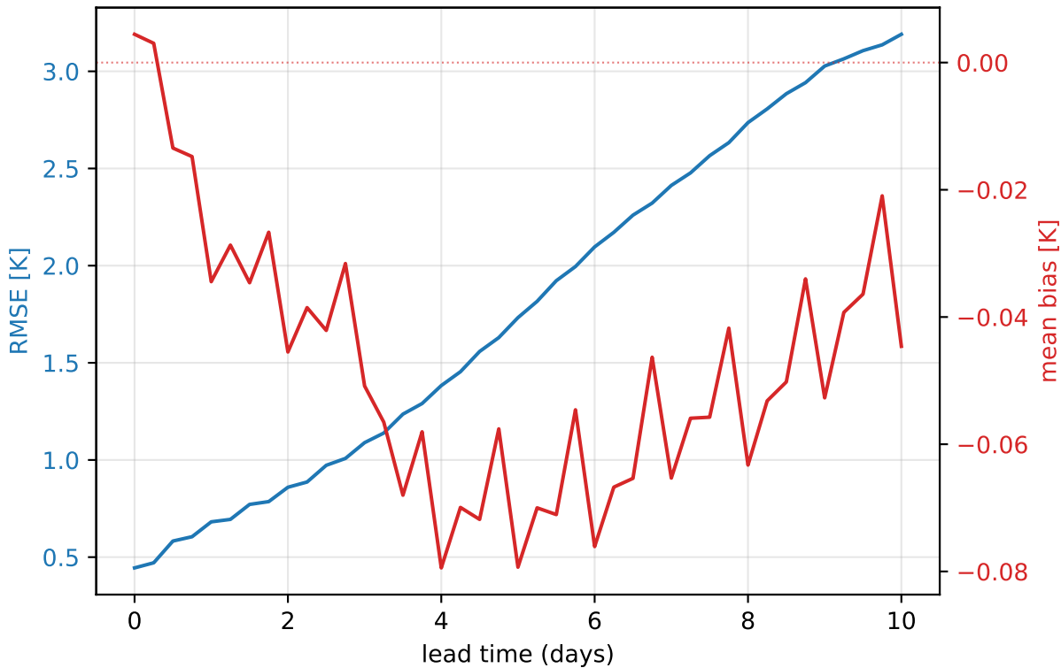
ERA5 2023 — 950 hPa temperature (global, mean of 30 daily inits)
