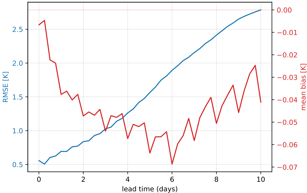
ERA5 2023 — 1000 hPa temperature (global, mean of 30 daily inits)
