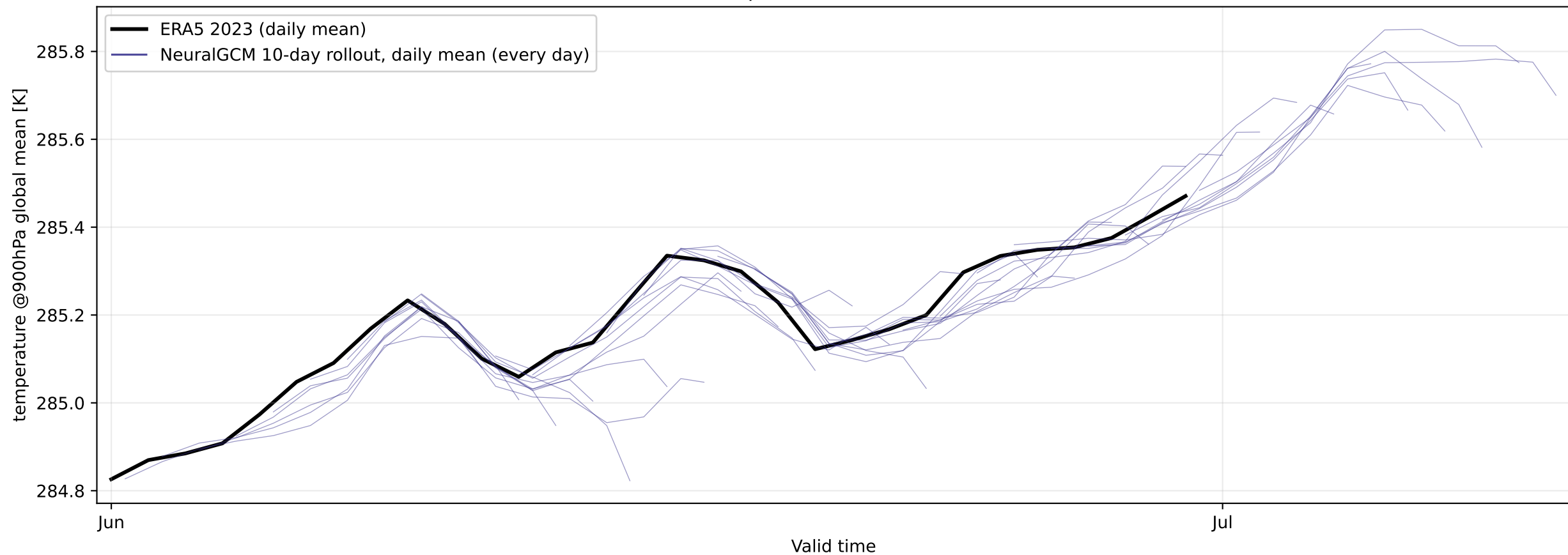
Global-mean temperature at 900 hPa — ERA5 2023
