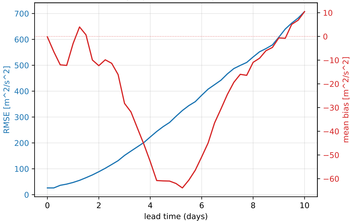
ERA5 2023 — 500 hPa geopotential (europe, mean of 31 daily inits)
