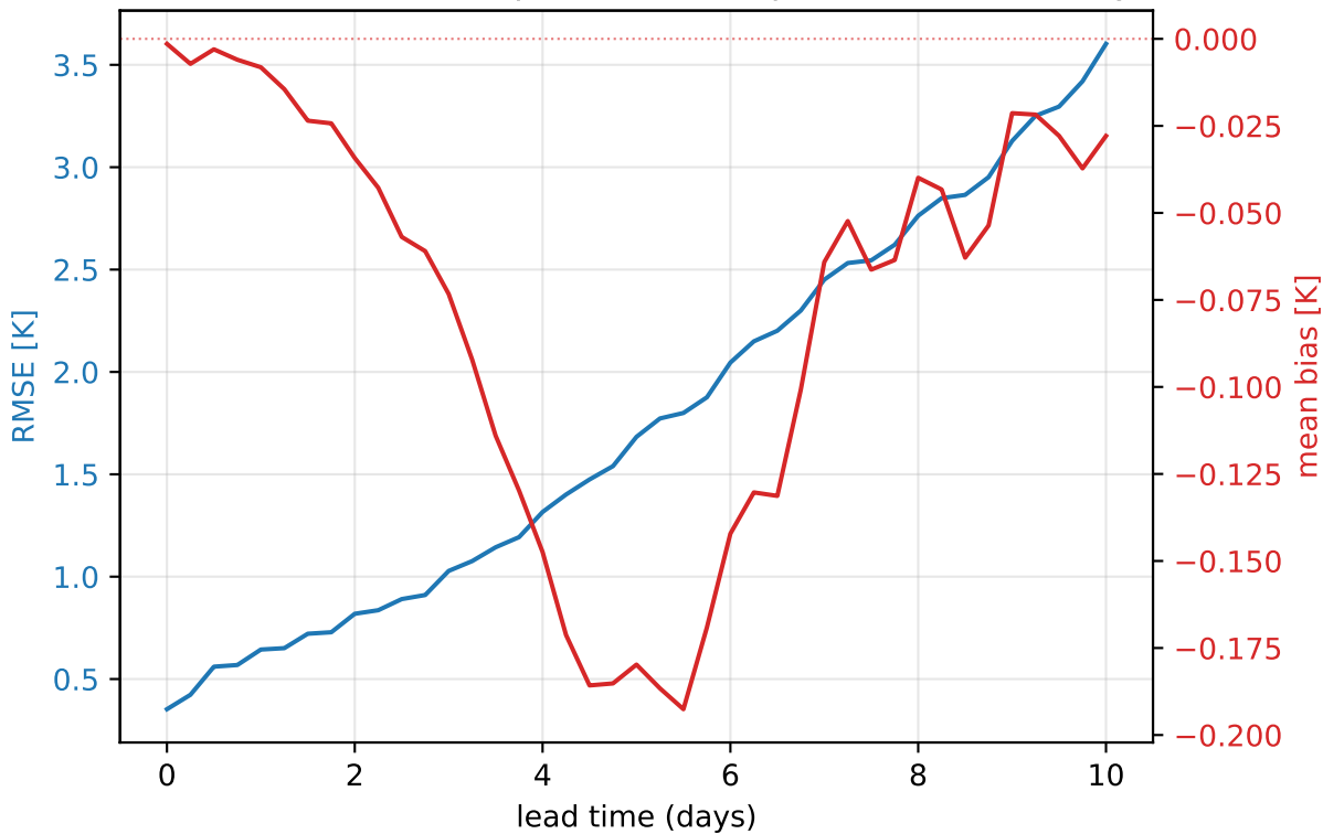
ERA5 2023 — 850 hPa temperature (europe, mean of 31 daily inits)
