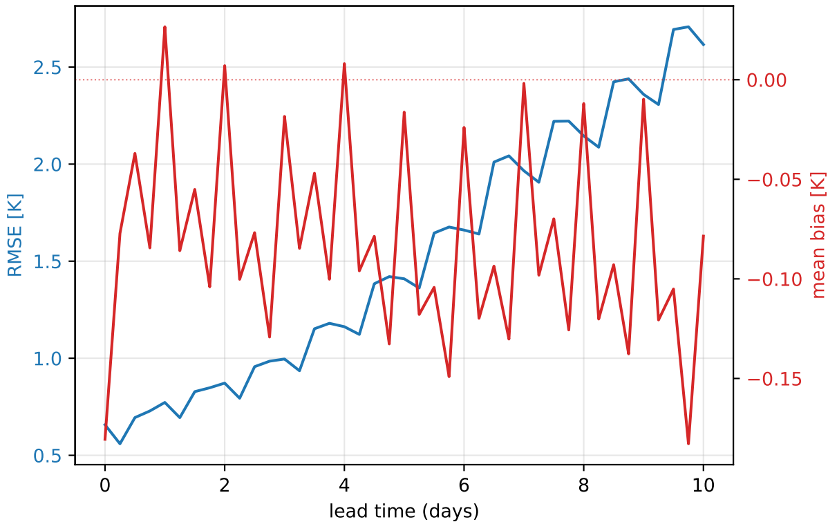
ERA5 2023 — 1000 hPa temperature (europe, mean of 31 daily inits)
