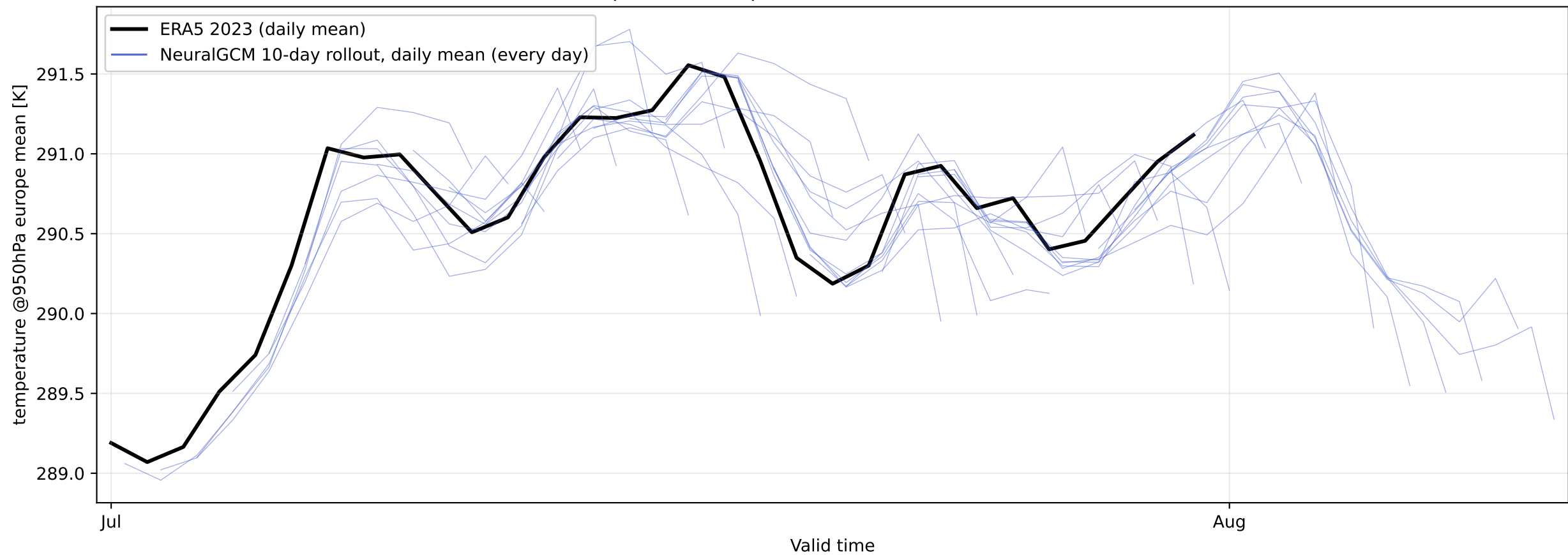
Europe-mean temperature at 950 hPa — ERA5 2023
